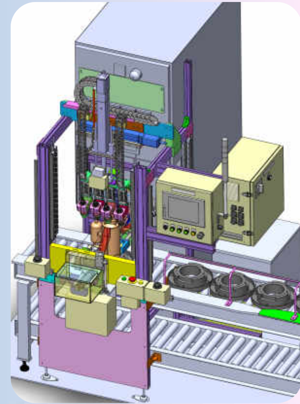
Resistance Check
