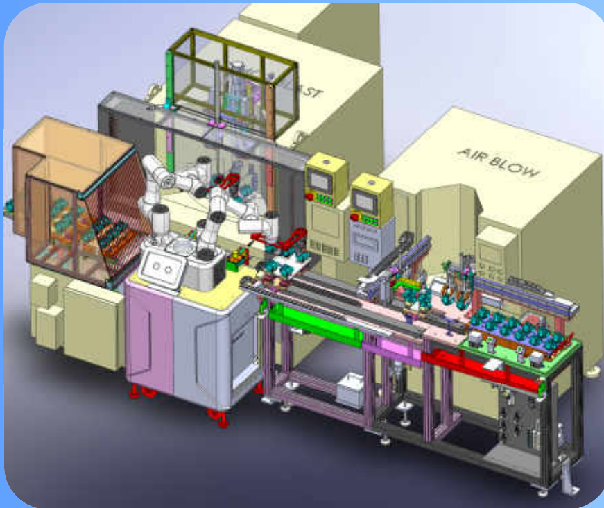
Auto Loader by Cobot
