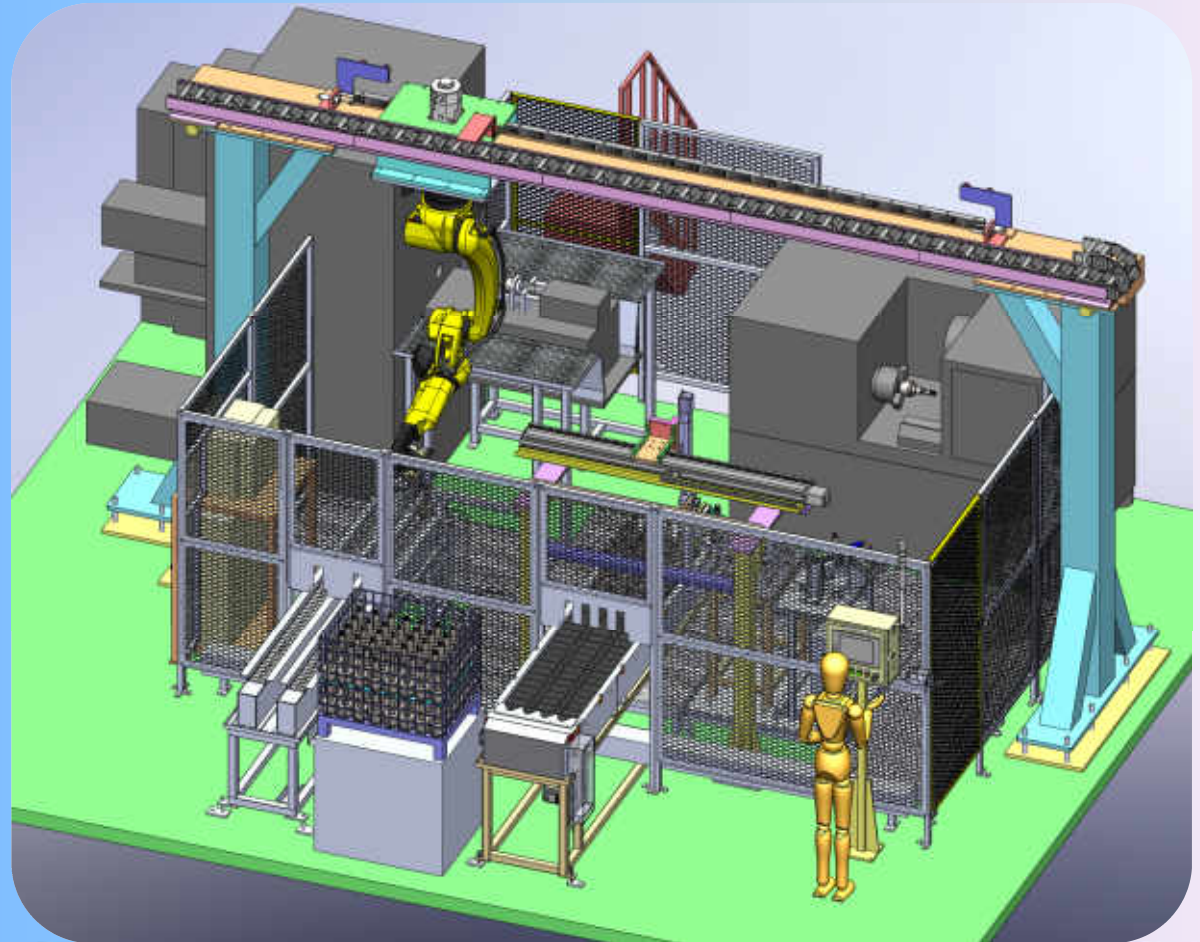
Fanuc Robot Loader,Dimension Check
