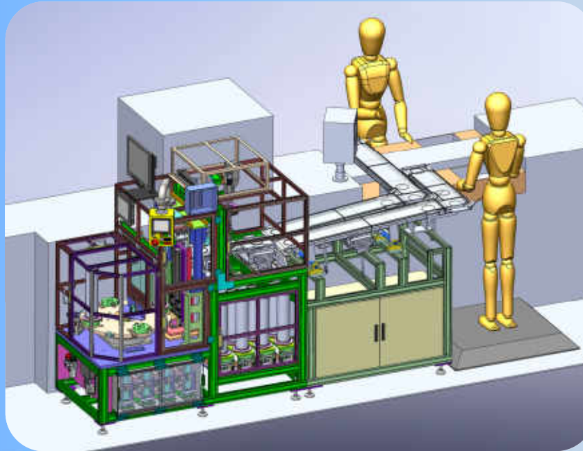
Camera Oring Counter
