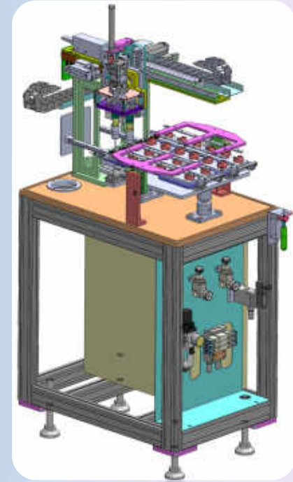
Lapping MC
