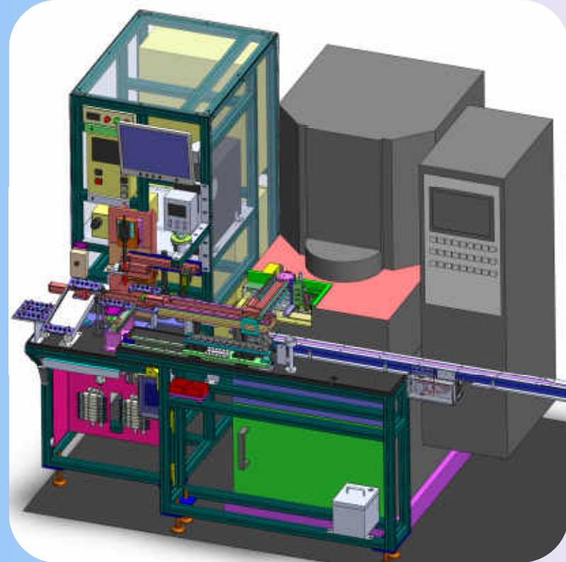
Auto Loader Conveyor
